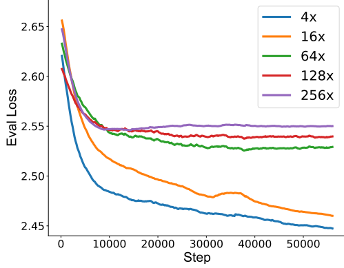
(a) Comparison across different compression rates (Lite)
