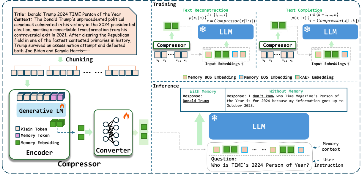
Figure 1: Overview of our PCC Framework. Given a long context, the compressor condenses the content into embedding-based memory slots for fast and accurate inference with an downstream LLM.
