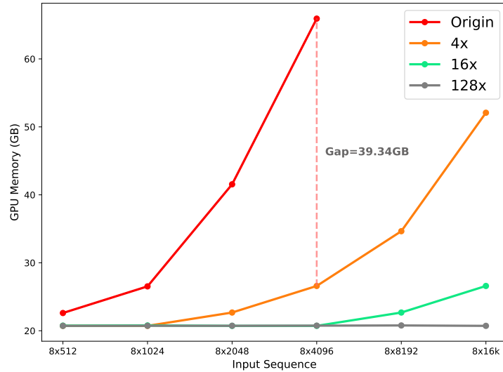
Figure A1: We compare the memory usage during inference between the original LLM method and the PCC method. The original LLM method, represented by Origin , runs out of memory (OOM) when the input text has a batch size of 8 and a length of 8192 tokens, exceeding 80 GB of GPU memory. In contrast, the PCC method maintains a much lower memory footprint under the same conditions.
