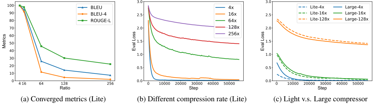
Figure 2: The converged metrics and pre-training curves for various configurations in the text reconstruction task.
