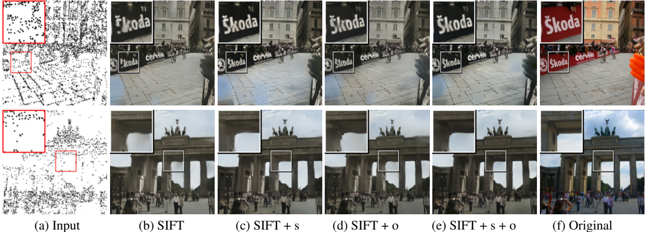
Figure 4: INVERTING SIFT FEATURES IN A SINGLE IMAGE: (a) 2D keypoint locations. Results obtained with (b) only descriptor, (c) descriptor and keypoint scale, (d) descriptor and keypoint orientation, (e) descriptor, scale and orientation. (f) Original image. Results from using only descriptors ( 2^{nd} column) are only slightly worse than the baseline ( 5^{th} column).
