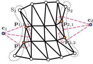
Figure 4: Boundary conditions for a self-supporting mesh. A convex boundary vertex (white circle) must be supported. In order to achieve horizontal equilibrium, each unsupported concave boundary vertex (orange circle) must possess a closed power cell, drawn in red. All cells along the same segment must share a common dual vertex (blue circle).
