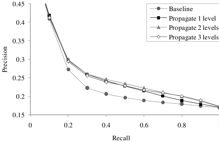
Fig. 3. Average precision vs. recall for 20 questions and all 189 employees. The interpolated precision at zero for all algorithms was approximately 0.58. To aid exposition, we adjust the scale of the y-axis to highlight the differences at all other recall levels.
