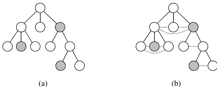
Fig. 1. (a) A sample organizational hierarchy. Links between nodes denote management relationships. (b) Links are added between peers (members with the same manager). By propagating scores from members with profiles (gray nodes) to those without (white nodes), more members in the organization can be covered. Additionally, the scores of members with profiles can be refined.
