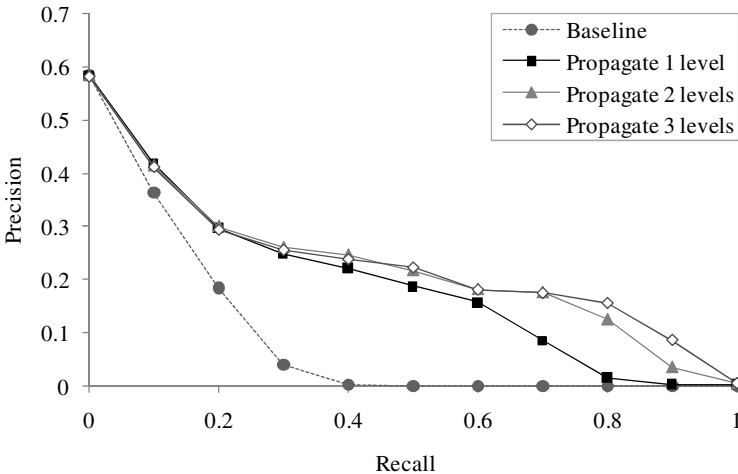
Fig. 2. The average precision (averaged across 20 questions) vs. recall for both the baseline and hierarchy-based algorithms
