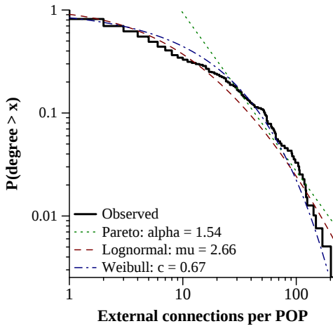
Fig. 16. A CCDF of the number of external adjacencies per POP. Some POPs are particularly important, while most have at least a few external connections.
