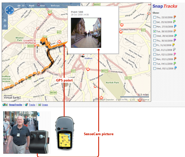
Figure 4. SnapTracks visualization.
