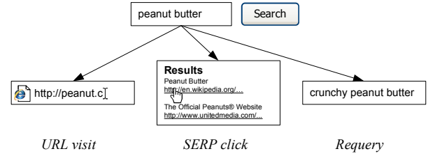
Figure 1. Post-query events
