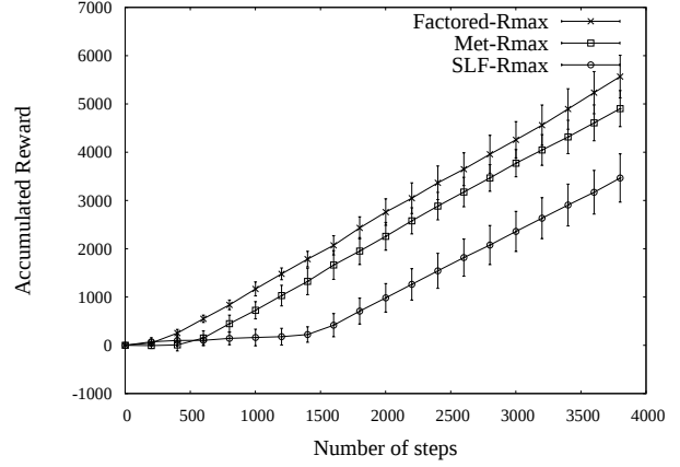
Figure 1. Cumulative reward on each timestep for the three algorithms on the Stock-trading domain: \text{Factored-}R_{\max} was given the DBN structure, while \text{Met-}R_{\max} and \text{SLF-}R_{\max} were not.
