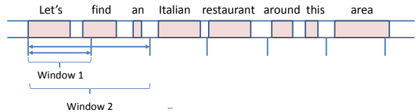
Figure 3: The window model
