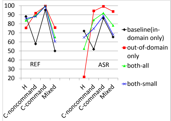
Figure 5: AD accuracies by utterance type
