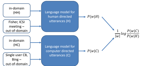
Figure 2: Language model-based score computation for addressee detection
