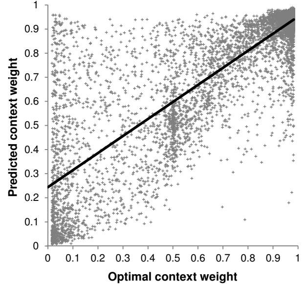
Figure 2. Predicted context weight vs. optimal context weight.
