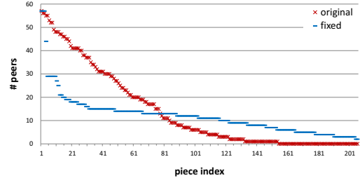
Figure 9: Piece distributions over peers when finishing 30% downloading.
