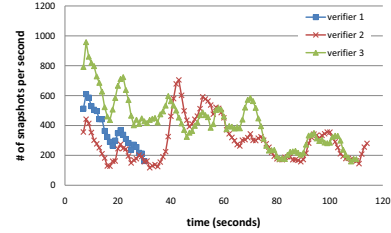
Figure 14: Load when verifier 1 fails at 30 th second.
