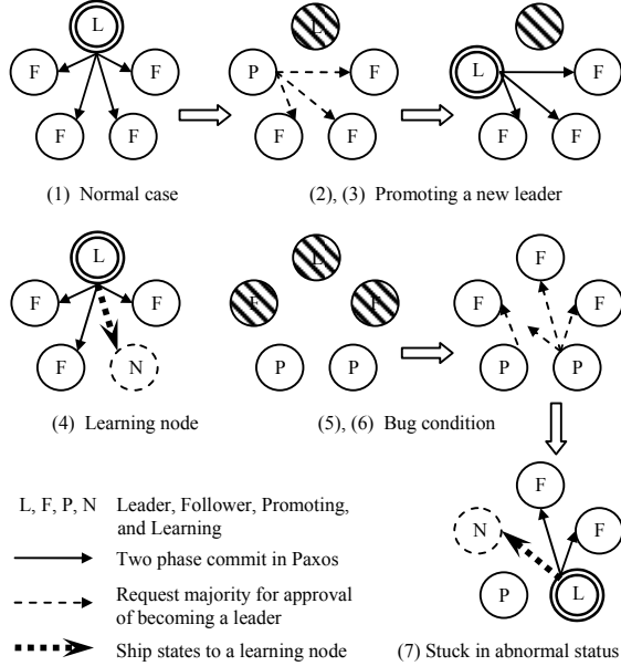
Figure 6: Leader election in Paxos implementation and the snapshots of states that lead to the bug.
